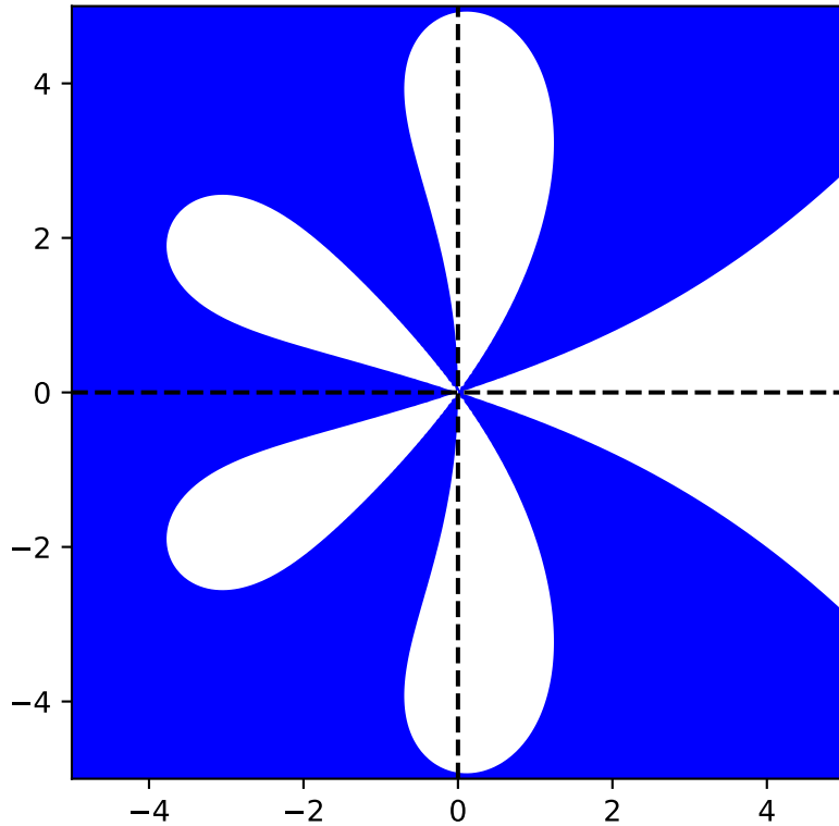
Order star for SSPRK(10,4)
