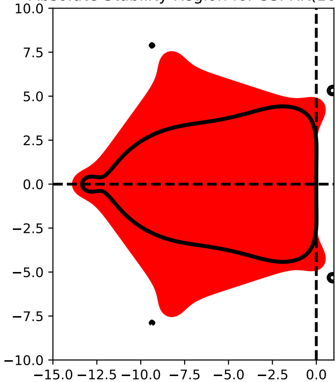
Absolute Stability Region for SSPRK(10,4)
